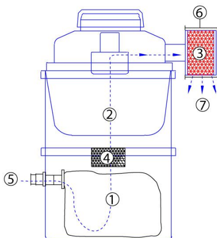
Luftstrømsdiagram for CWR-10 EX CV containment-system
